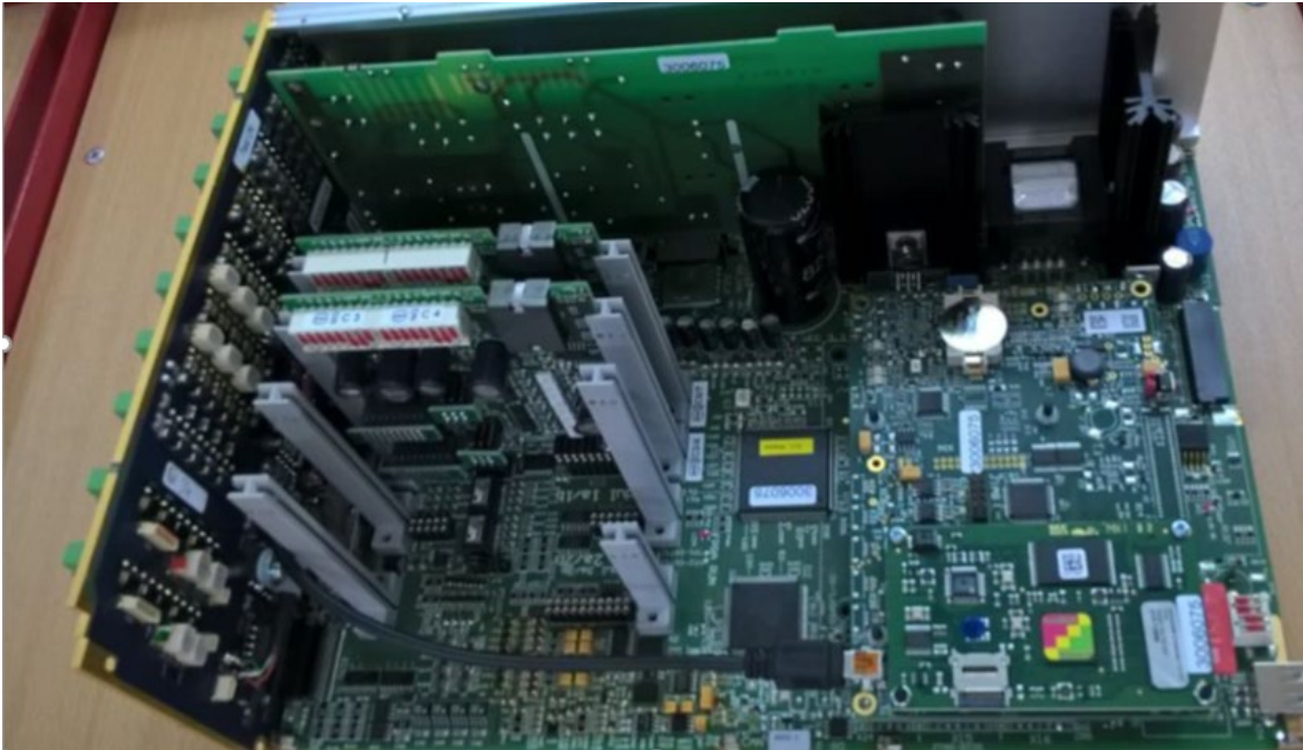
Fig. 8.21: Slot for the option card with COM 6 and 7 of the ERZ 2000-NG
