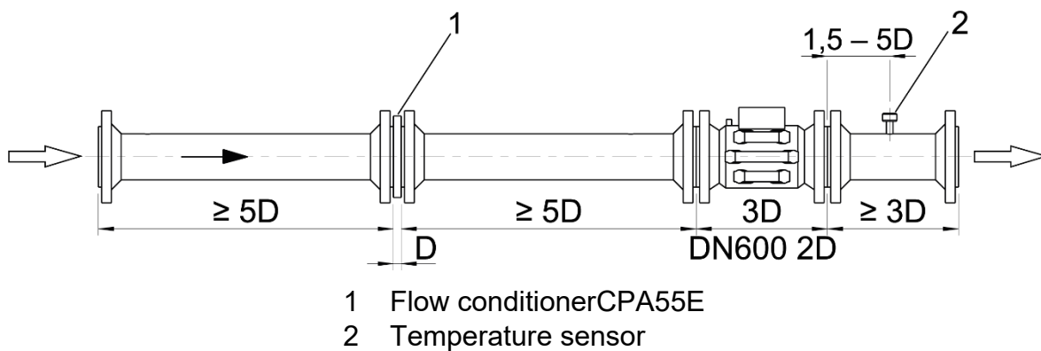
Fig. 7.6: Unidirectional operation – compact installation with flow conditioner CPA55E
