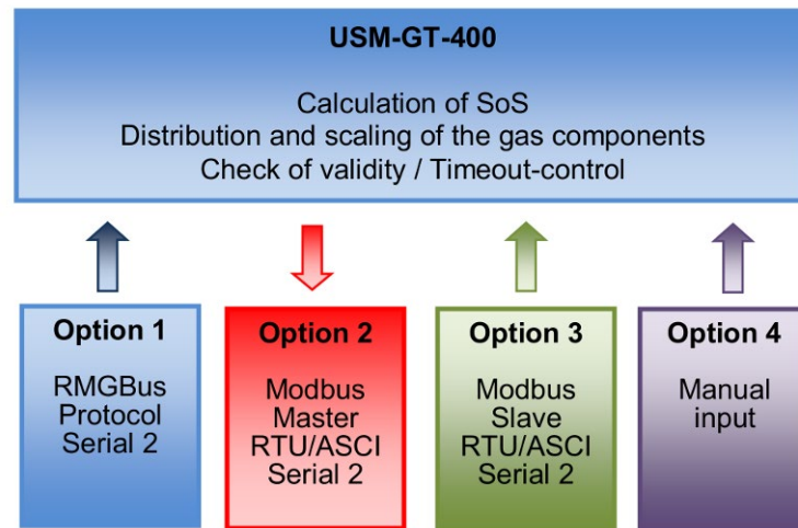
Fig. 4.3: Import of gas composition data
