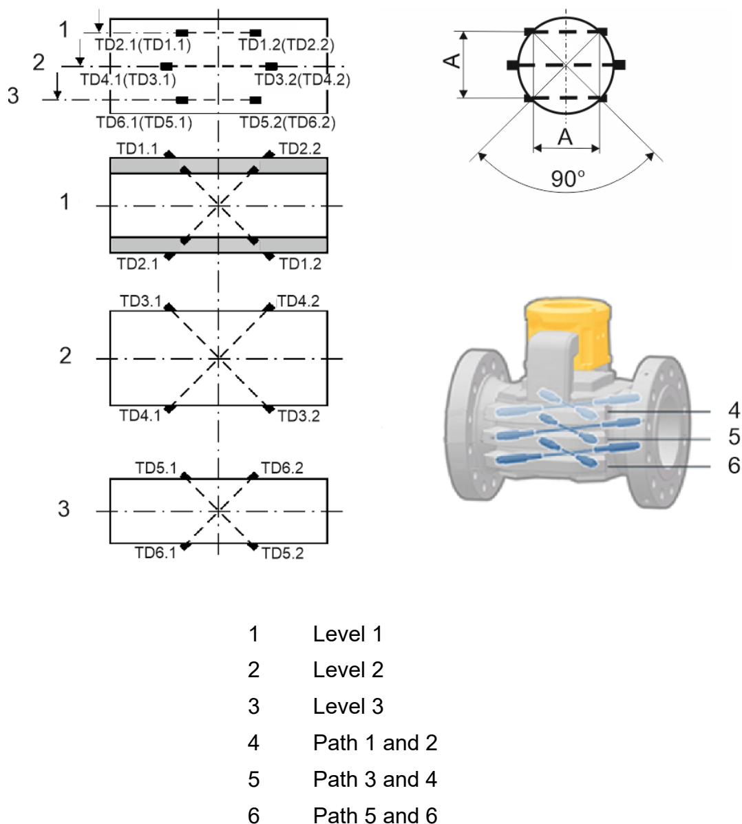
Fig. 3.5: Transducer paths and levels of the ultrasonic gas meter
