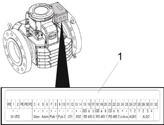
1 Terminal Connections
