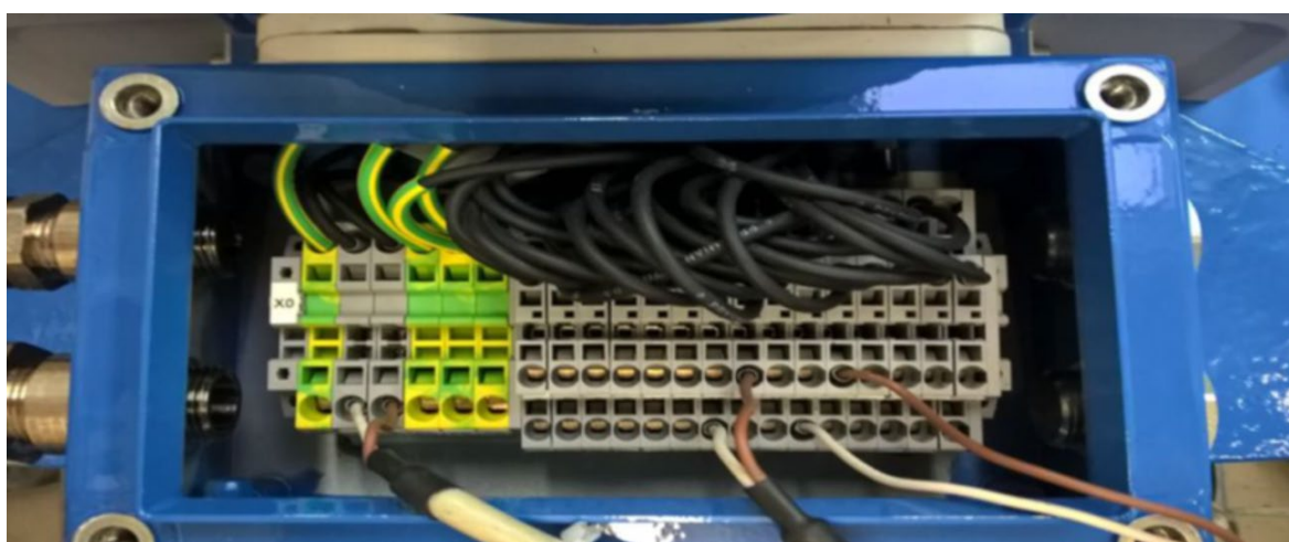
Fig. 8.19: Connection of the RS 485-2 (22 +, 23 -) at the USM GT400
