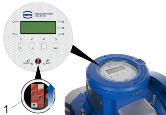
1 Calibration switch
