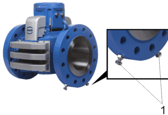
1 Retaining bolts
