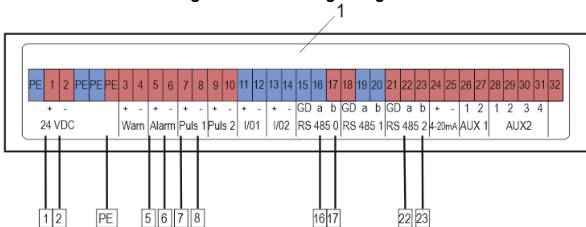
1 Terminal connections
