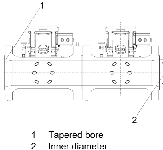
Fig. 7.10: Face-to-Face Installation
