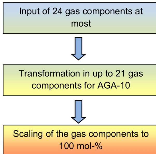
Fig. 4.7: Sequence of gas components treatments
