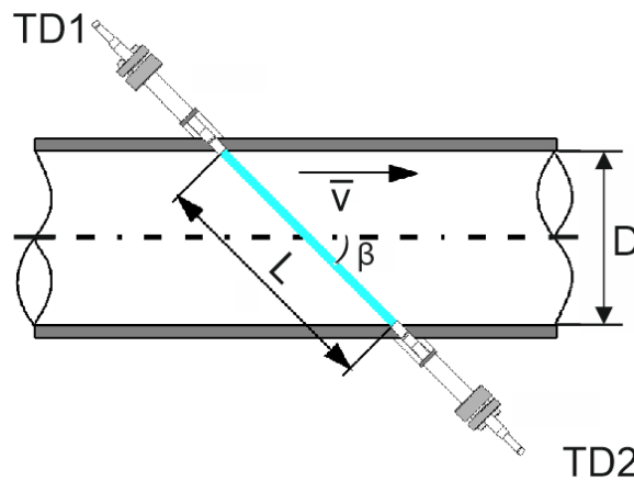
Fig. 4.1: Two sensors form one path for the measurement
