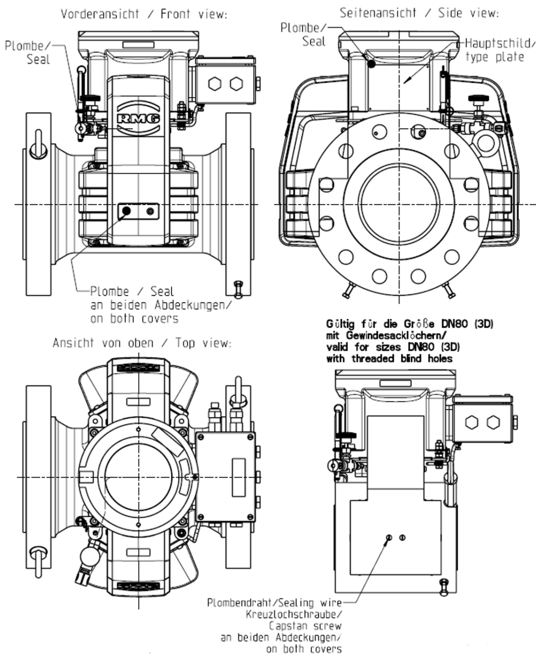
Fig. 13.11: Devices DN 80 (3"), DN 100 (4") and DN 150 (6")
