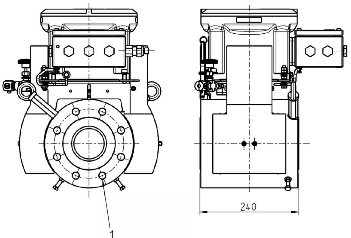
Fig. 13.7: Weights and dimensions DN80
