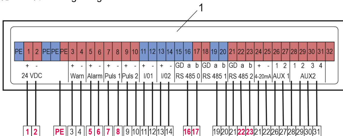
1 Terminal connections
