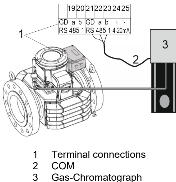
Fig. 4.4: Terminal connections
