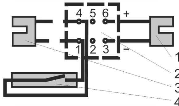
Figure 10: Connector pin assignments for the HF 1 pulse transmitter
