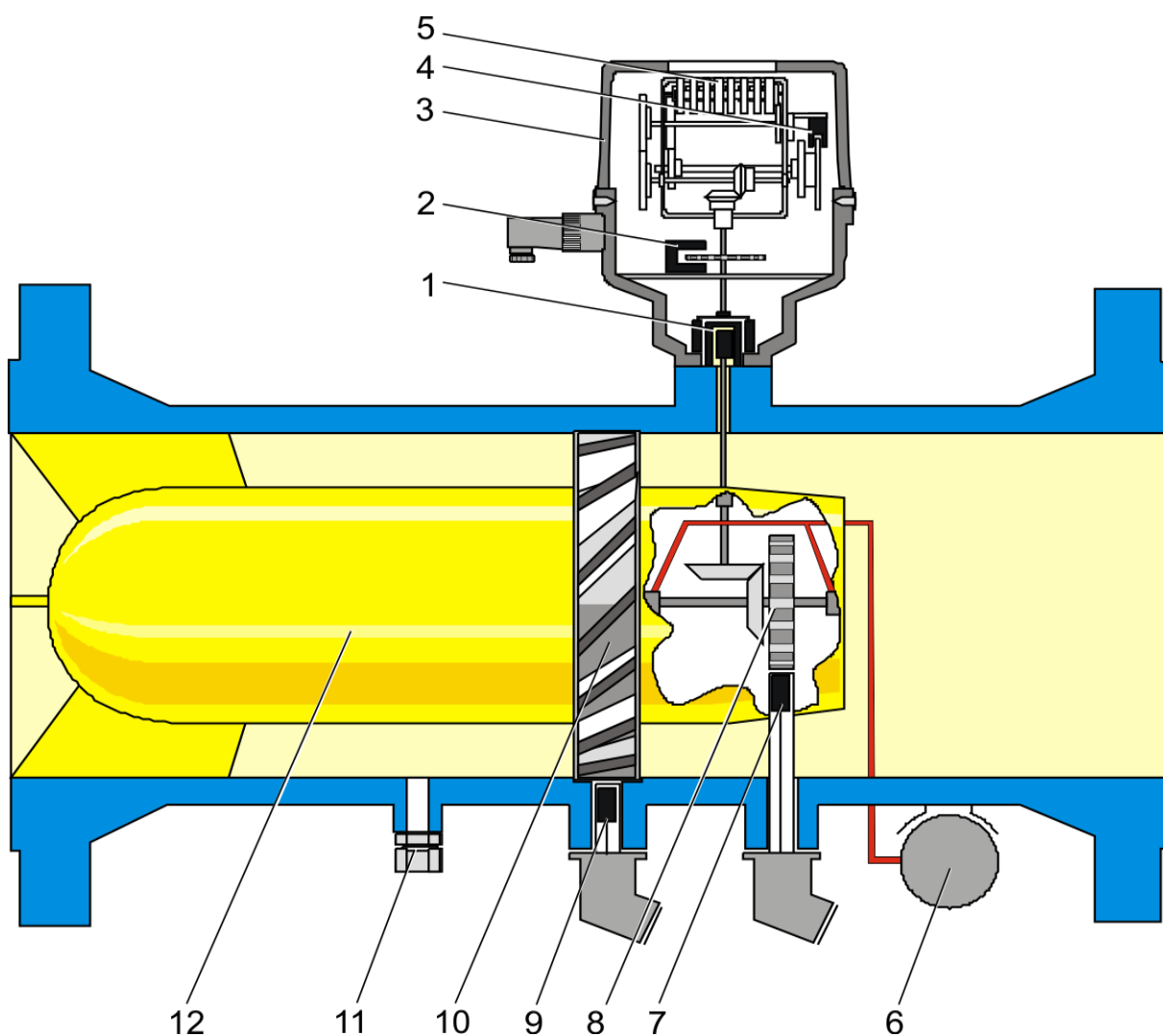
Figure 12: Sectional drawing of a turbine meter
