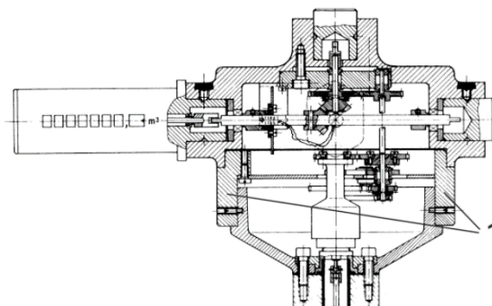
Figure 6: Type “D” meter head
