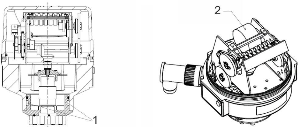
Figure 3: Type “F” meter head
