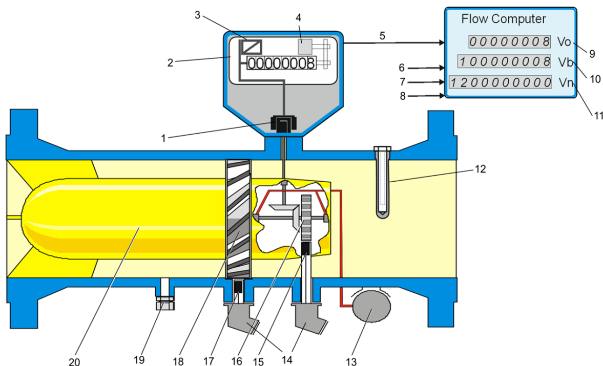
Figure 1: Sectional drawing of a turbine meter
