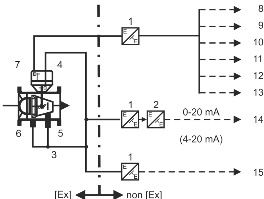
Figure 9: Connection options of the TRZ 03
