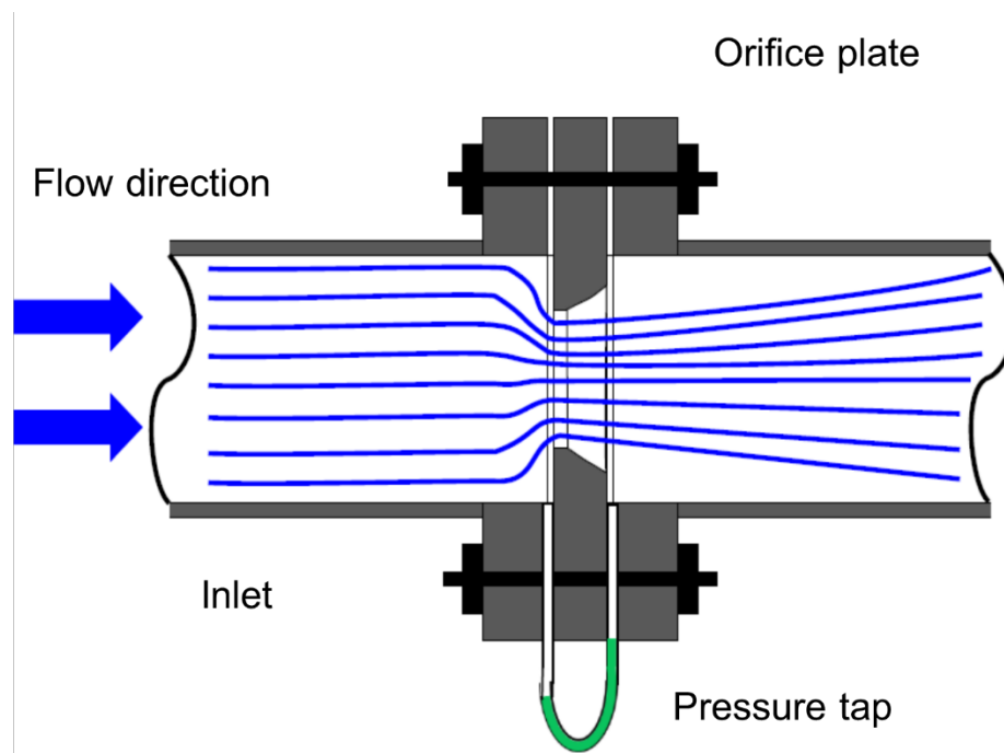
Figure 184: Orifice plate flow rate meter measuring principle
