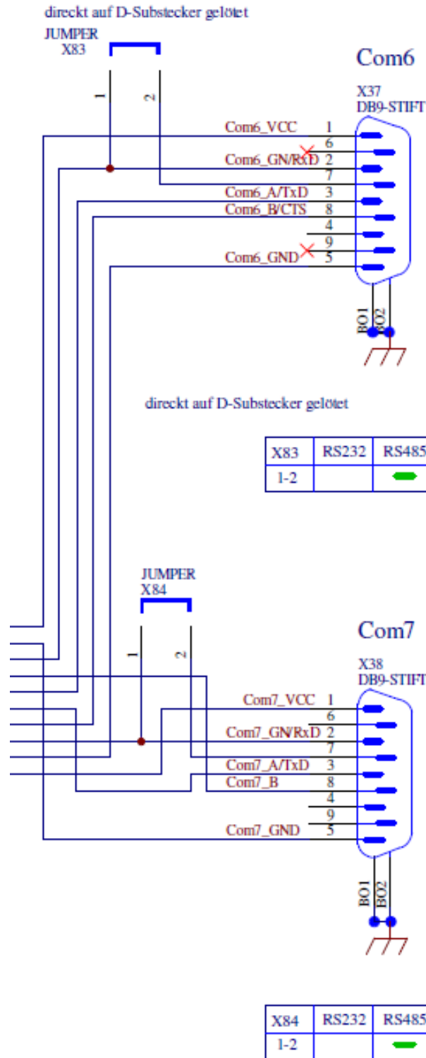
Figure 170: Jumper COM6/7 on the rear wall
