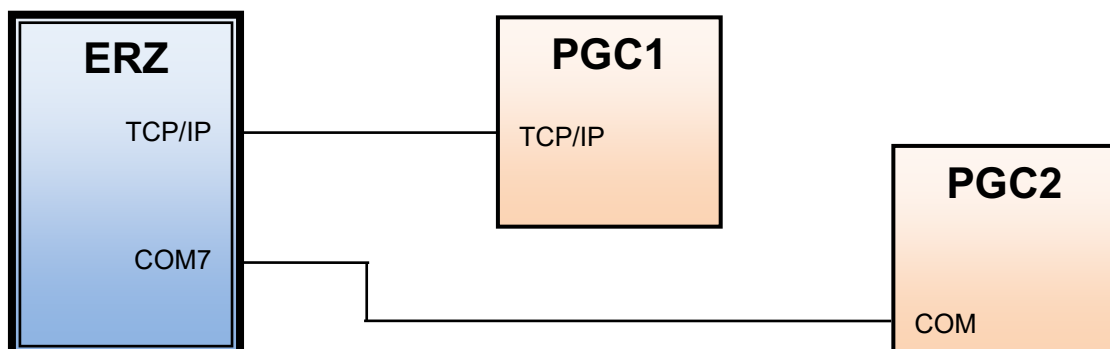
Figure 109: "Mixed" connection of PGCs (gas analysis)
