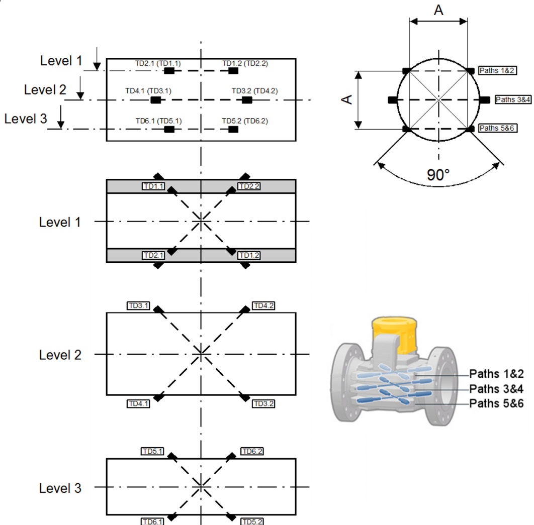
Figure 144: Ultrasonic measuring paths
