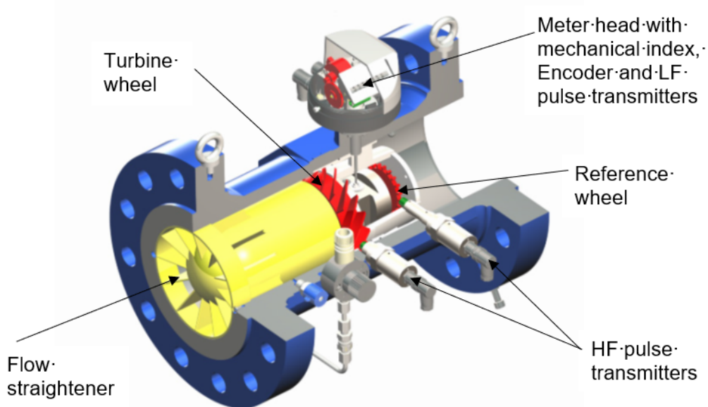
Figure 140: Turbine meter sectional drawing
