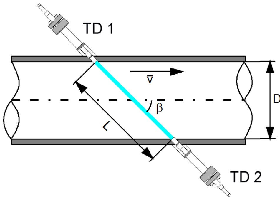
Figure 143: 2 Transducers form a path for the measurement
