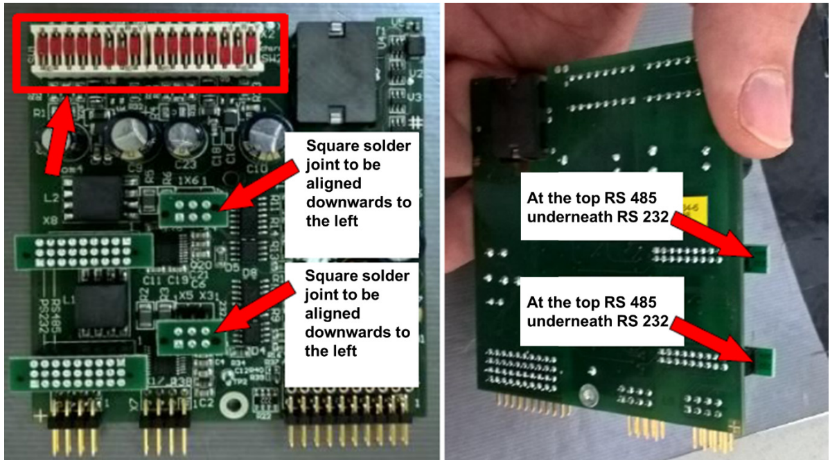
Figure 166: Option board configuration for use as COM6 and 7
