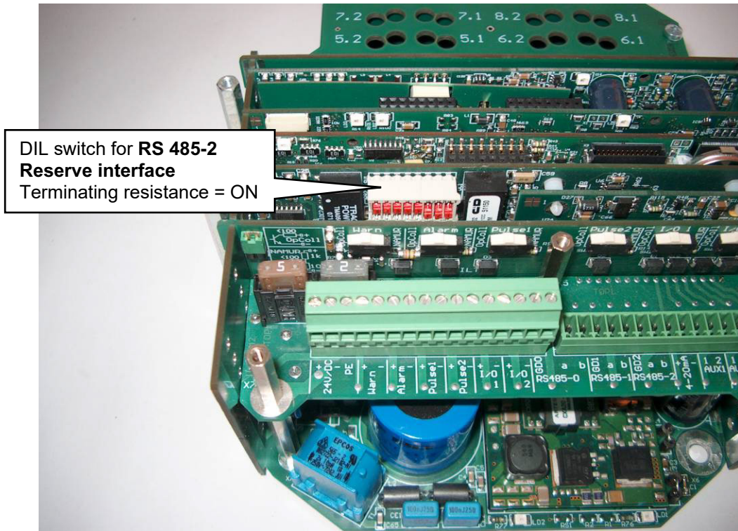
Figure 277: USE-09 Electronics of the USM-GT400 or USZ 08
