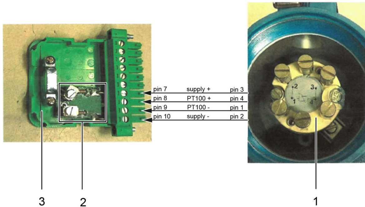
Figure 89: Connection of a PT100 without series resistors to a connector plug
