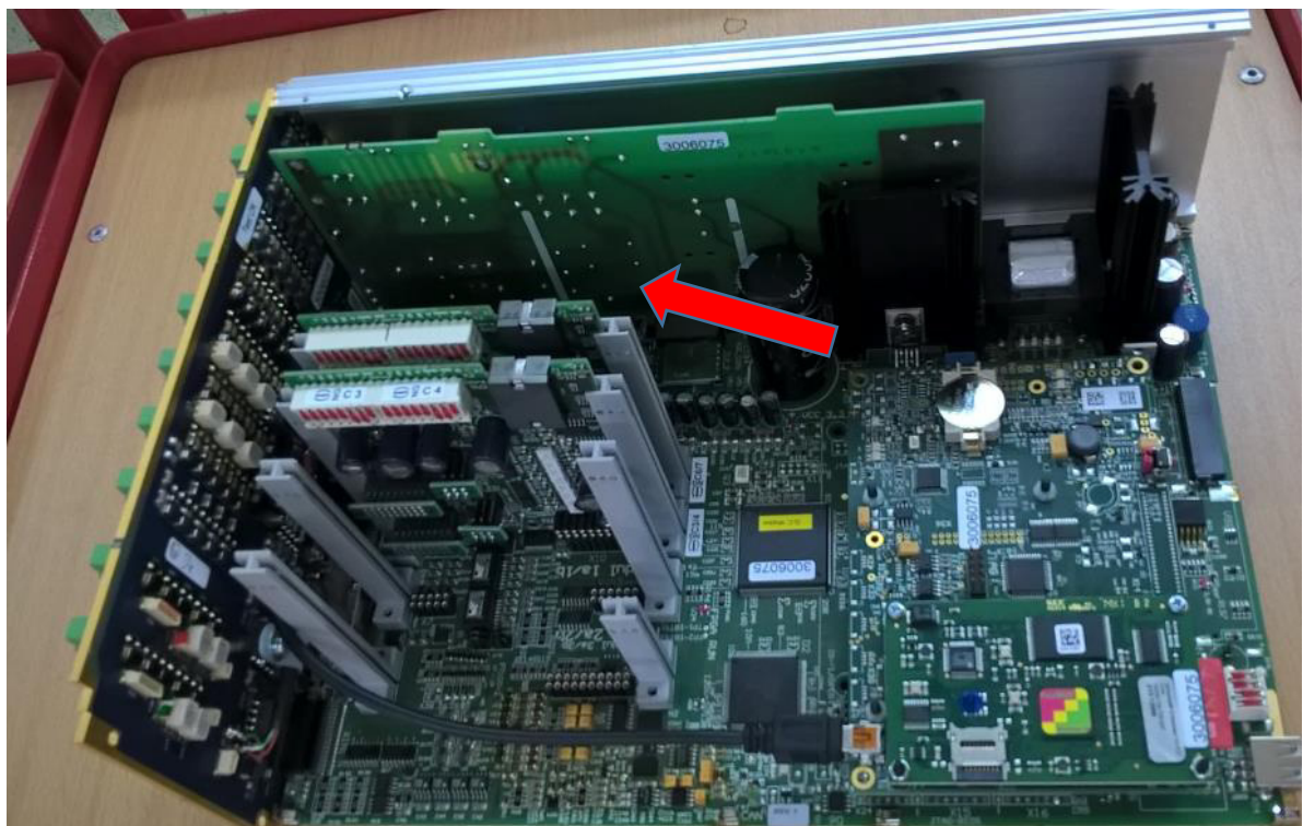
Figure 167: Slot of the option board for COM6 and 7
