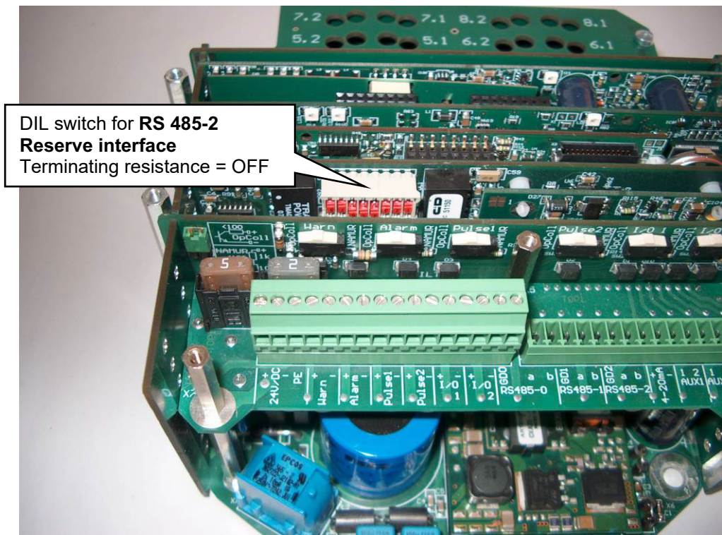
Figure 278: USE-09 Electronics of the USM-GT400 or USZ 08
