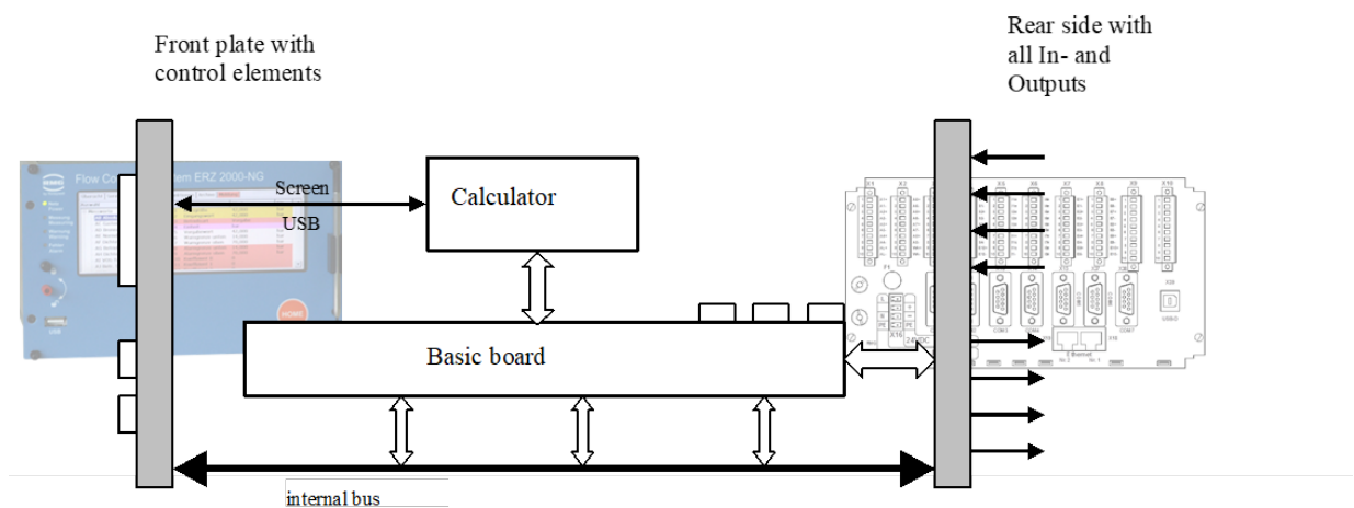
Figure 2: System configuration overview
