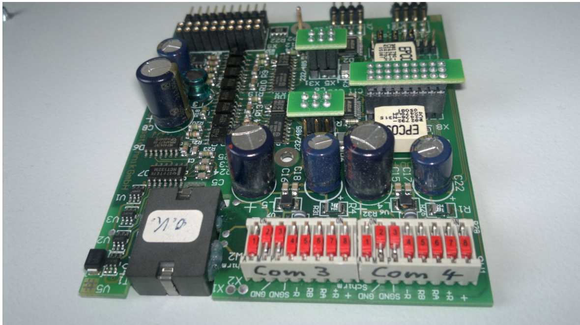
Figure 105: DIL switches of COM 3 and COM 4
