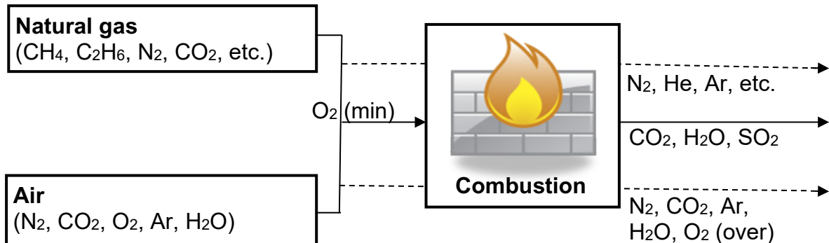
Figure 215: Combustion of natural gas with air
