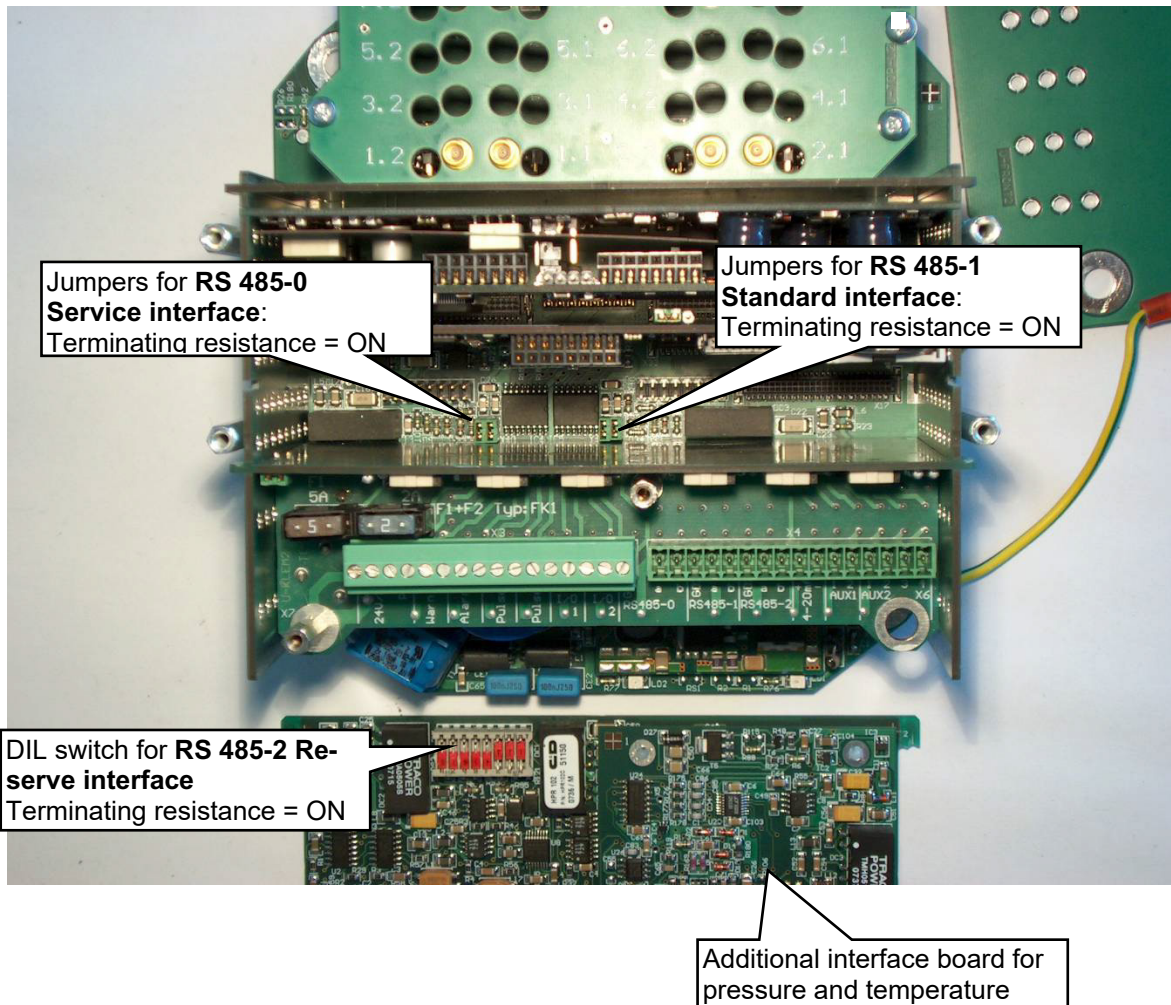
Figure 276: USE-09 Electronics of the USM-GT400 or USZ 08
