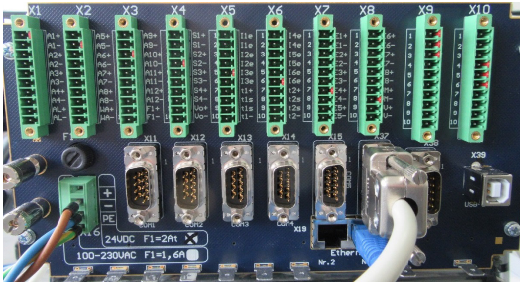
Figure 164: Connection of the Modbus interface of the USM to COM 6
