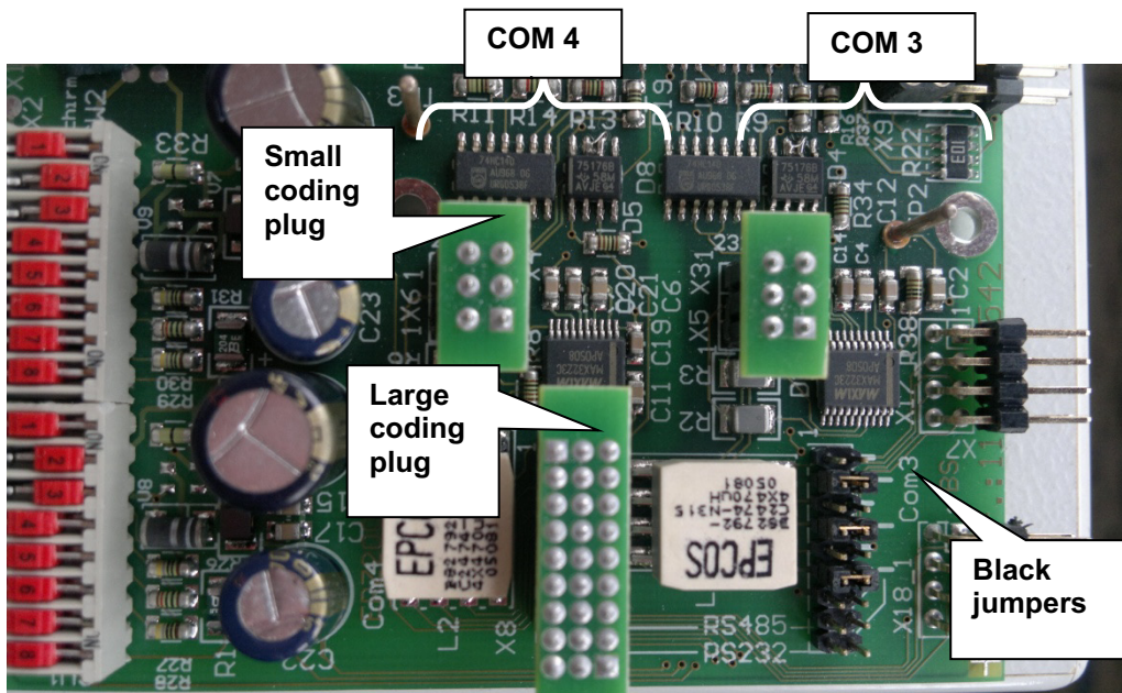
Figure 230: Coding plugs and bridges of COM 3 and COM 4
