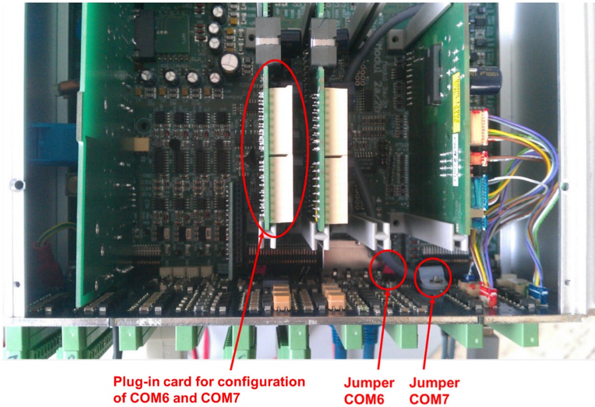
Figure 168: Jumpers for COM6 and COM7 on the rear wall
